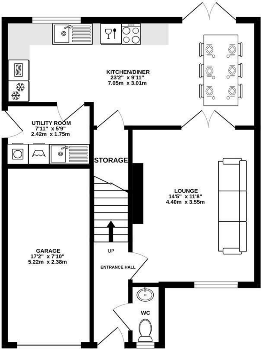
TOTAL FLOOR AREA : 1217 sq.ft. (113.1 sq.m.) approx.
